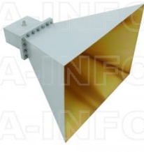
LB-975-15-C-7/16F Standard Gain Horn Antenna 0.75-1.12GHz 15dB Gain 7/16(DIN) Female
